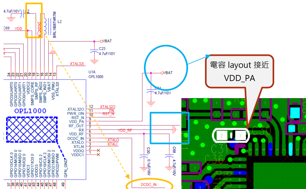
Figure 6. RF 电源电路 1
