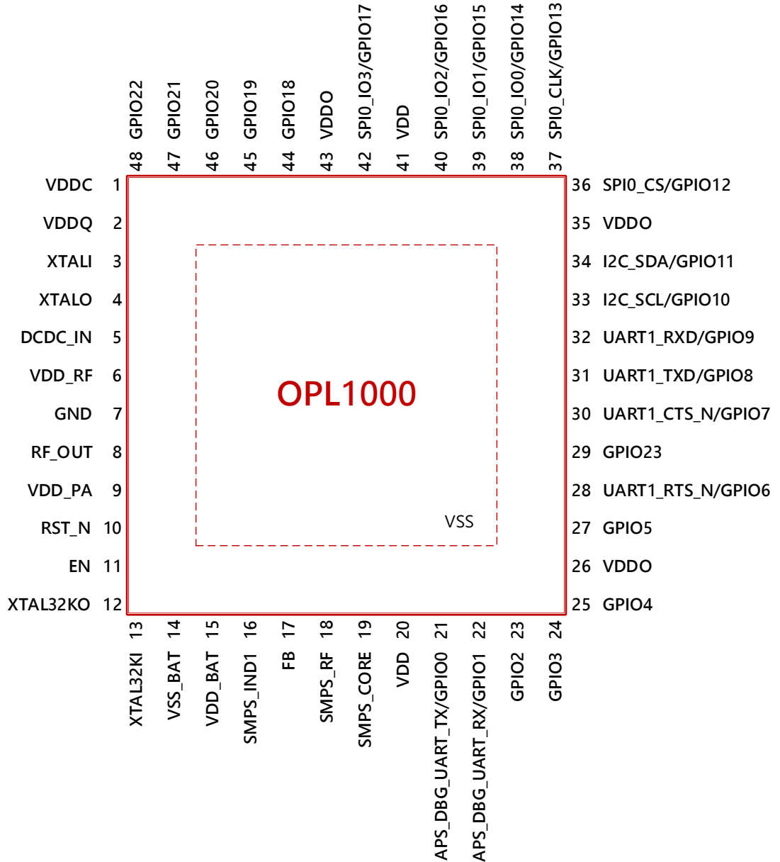
Figure 2. OPL1000 Pin Layout
