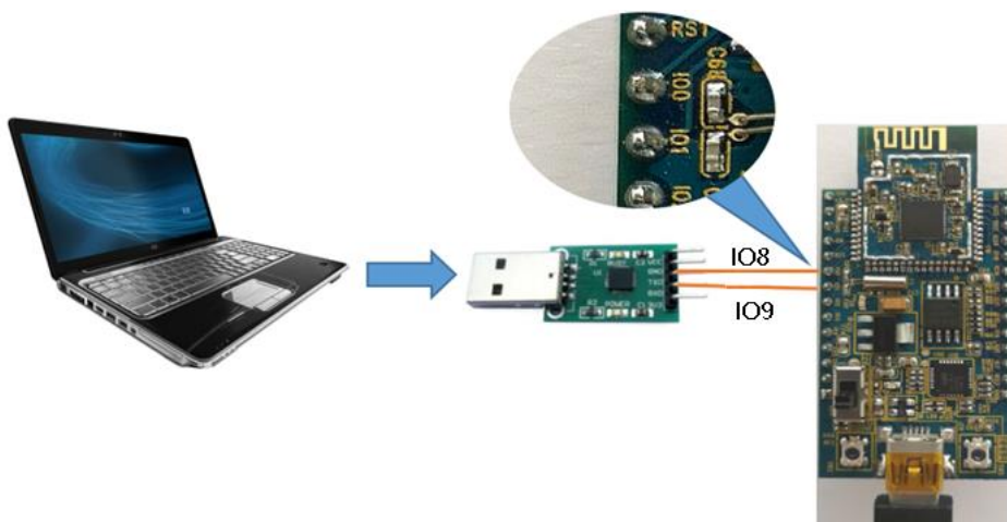
Figure 3: DevKit 接线图
